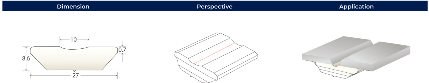
(3) Lascentrum Welding stone SB02
