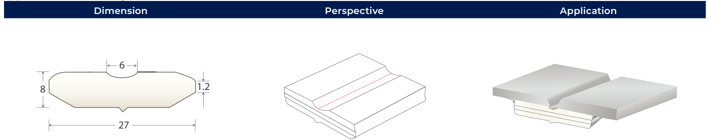
(2) Lascentrum Welding stone SB01A
