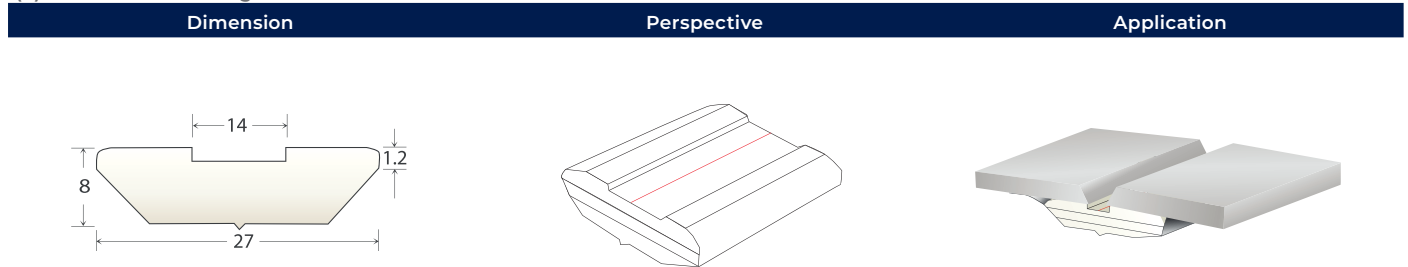
(4) Lascentrum Welding stone SB03
