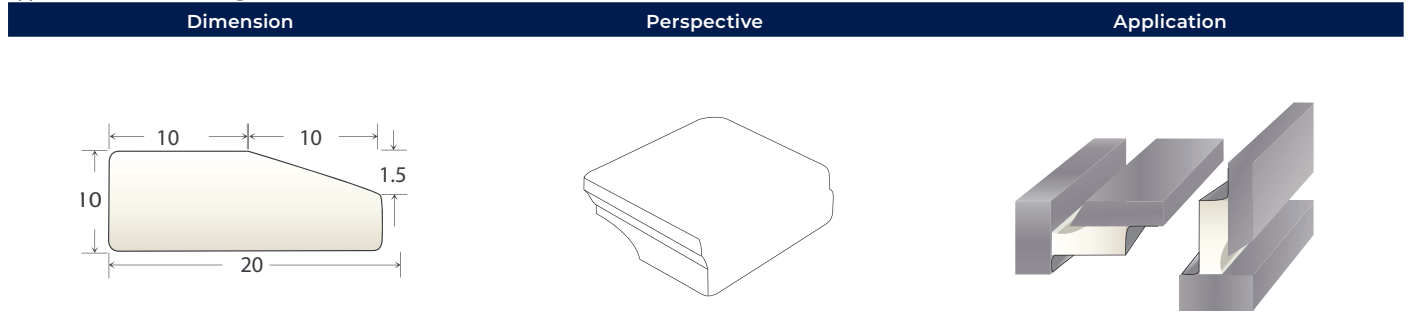
(1) Lascentrum Welding stone SB12
