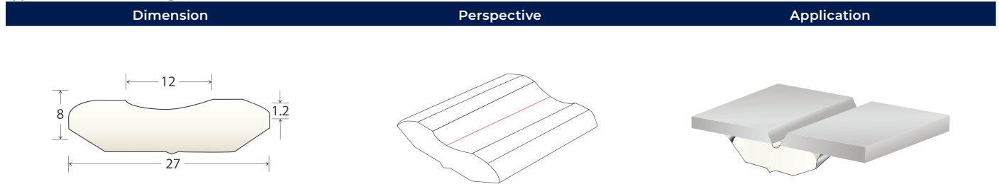
(1) Lascentrum Welding stone SB01
